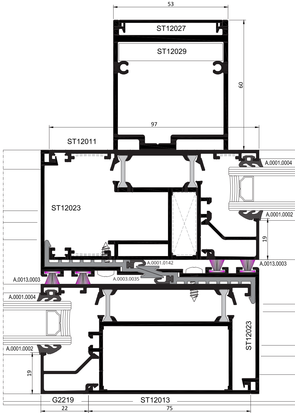
MONORAIL KALDIR-SÜR DETAYI MONORAIL LIFT & SLIDE DETAIL
