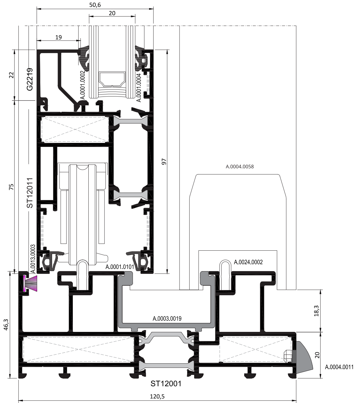
KALDIR-SÜR DETAYI LIFT & SLIDE DETAIL
