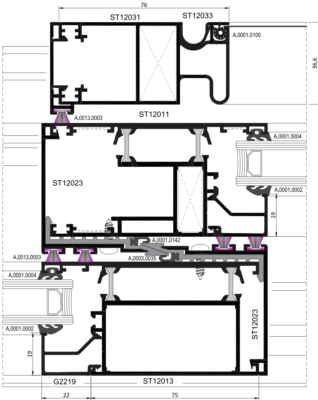
MONORAIL KALDIR-SÜR DETAYI MONORAIL LIFT & SLIDE DETAIL
