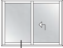
35 MONORAIL KALDIR-SÜR DETAYI MONORAIL LIFT & SLIDE DETAIL
