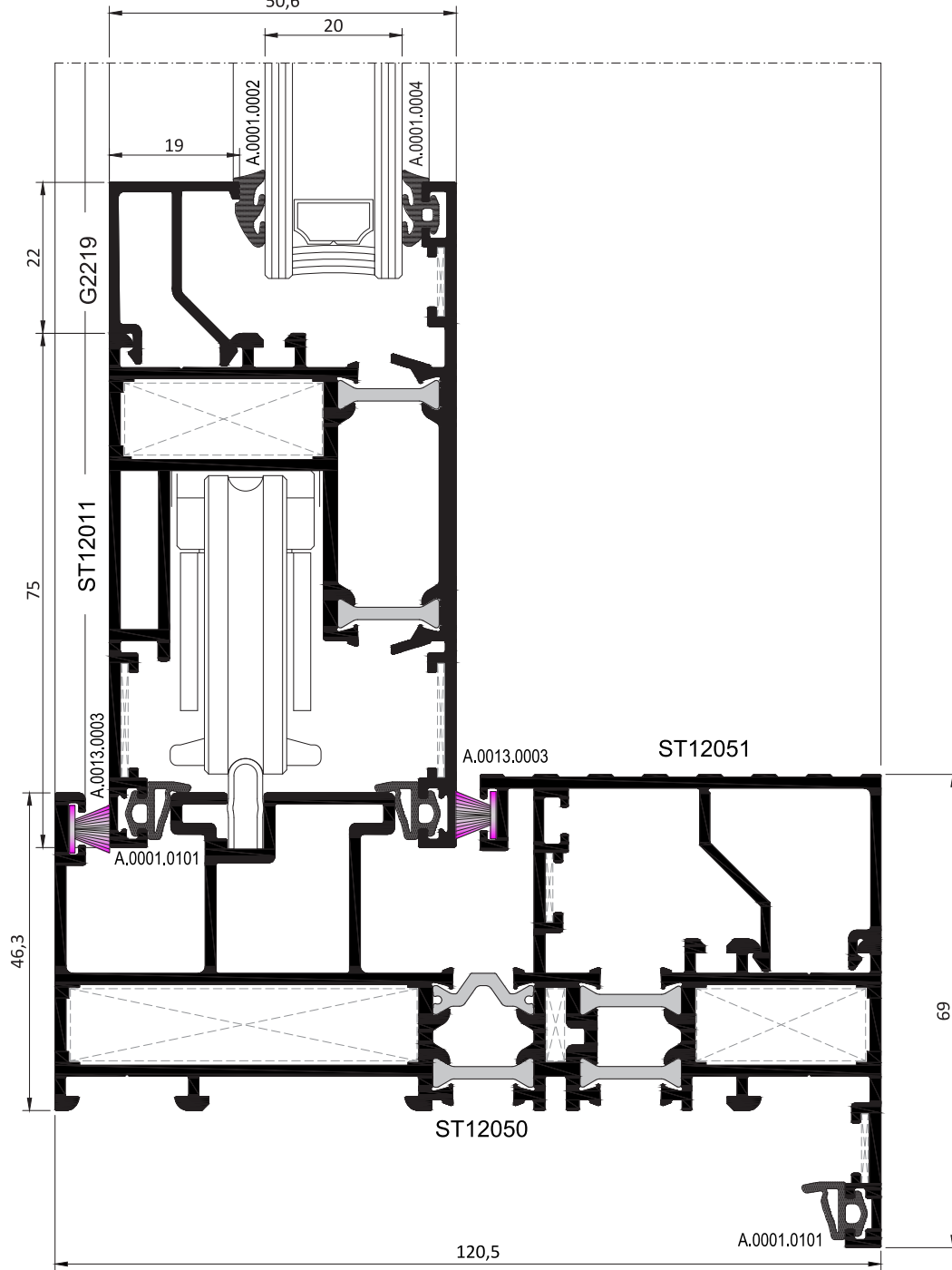
MONORAIL KALDIR-SÜR DETAYI MONORAIL LIFT & SLIDE DETAIL
