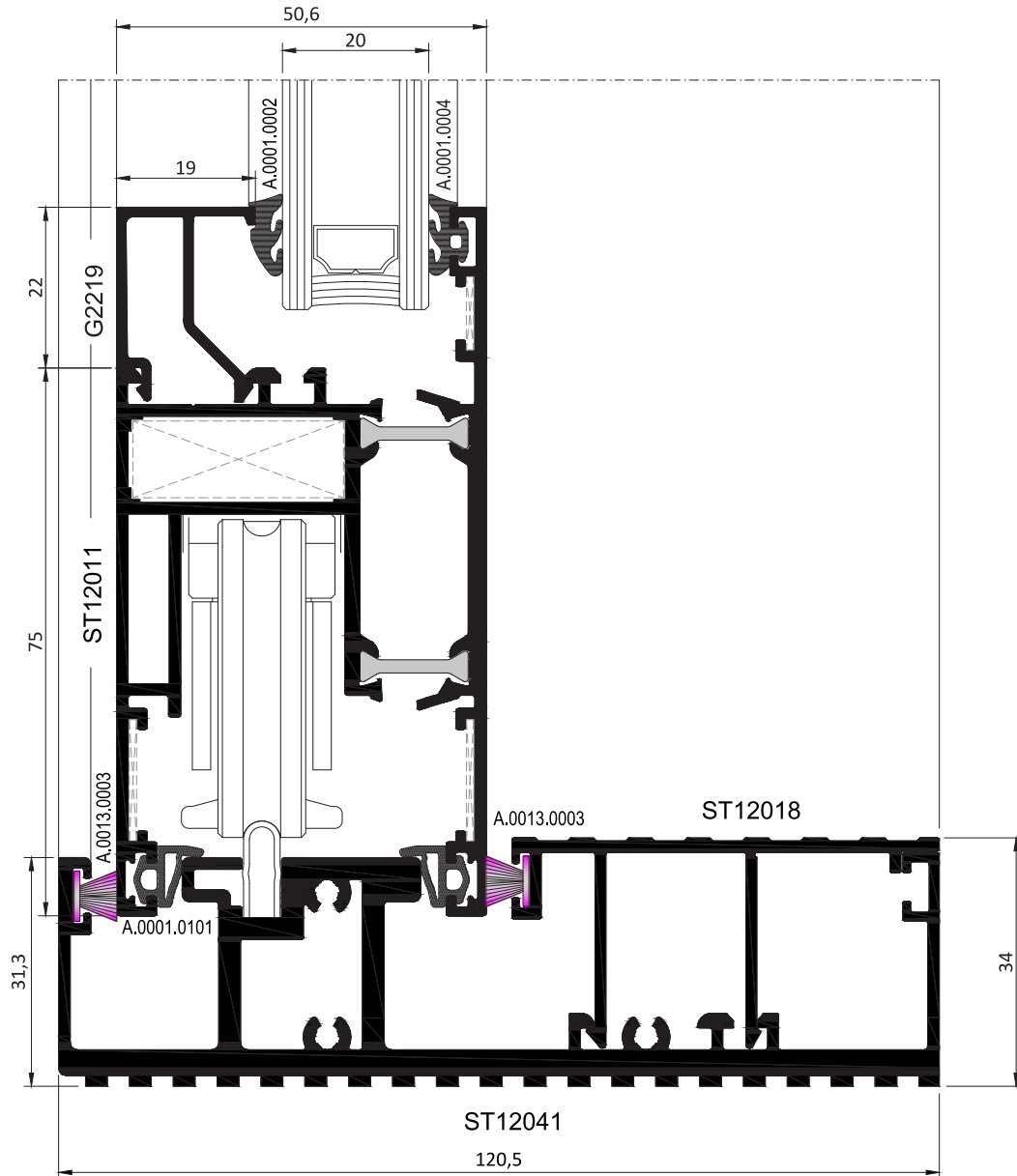
KALDIR-SÜR DETAYI LIFT & SLIDE DETAIL
