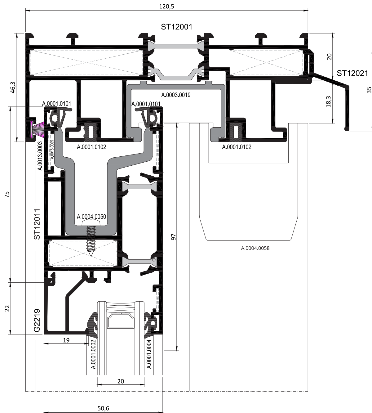
KALDIR-SÜR DETAYI LIFT & SLIDE DETAIL
