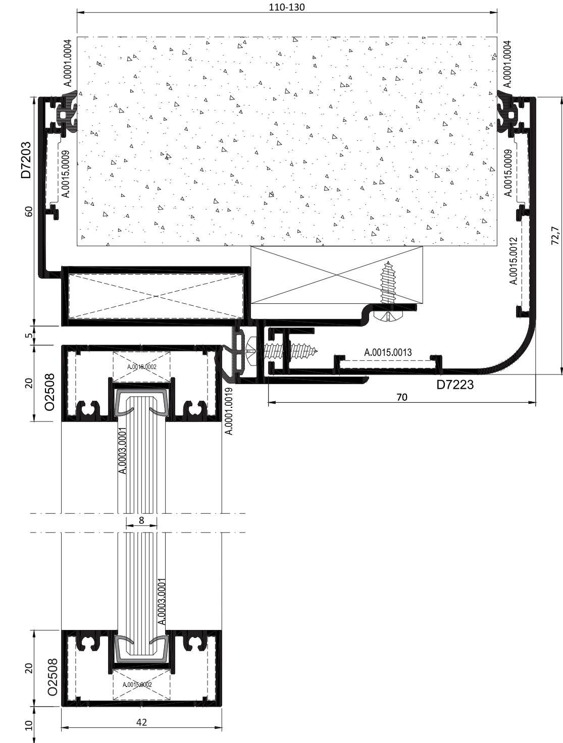
ALÜMİNYUM PERVAZLI KAPI SİSTEMİ - KANAT KESİTİ DOOR SYSTEM WITH ALUMINUM SILL- VENT SECTION
