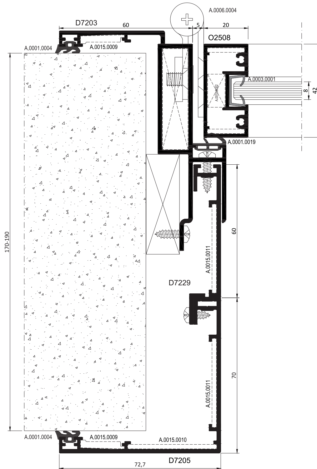
ALÜMİNYUM PERVAZLI KAPI SİSTEMİ - KANAT KESİTİ DOOR SYSTEM WITH ALUMINUM SILL- VENT SECTION
