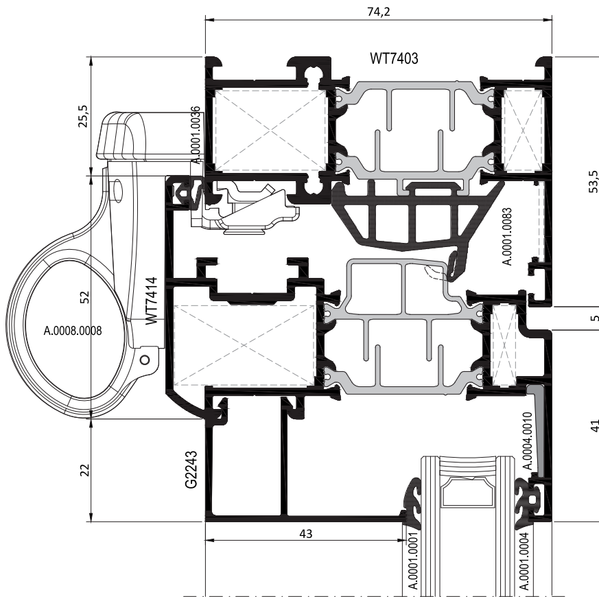
VASİSTAS AÇILIM PENCERE DETAYI BOTTOM HUNG OPENING DETAIL
