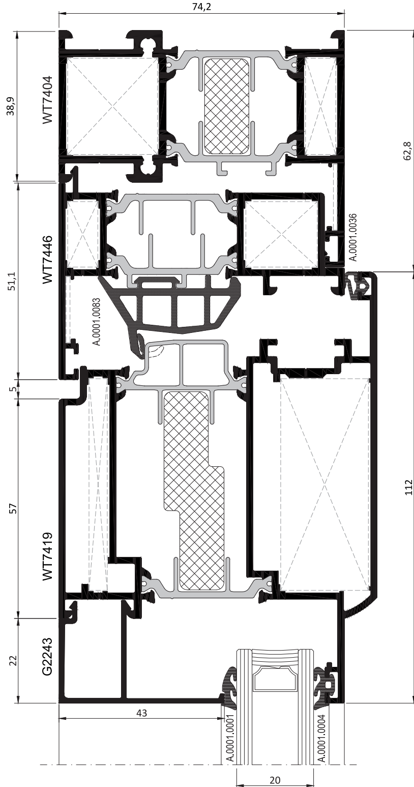
DIŞA AÇILIM BİNLİ KAPI DETAYI OUTWARD OPENING DOOR DETAIL
