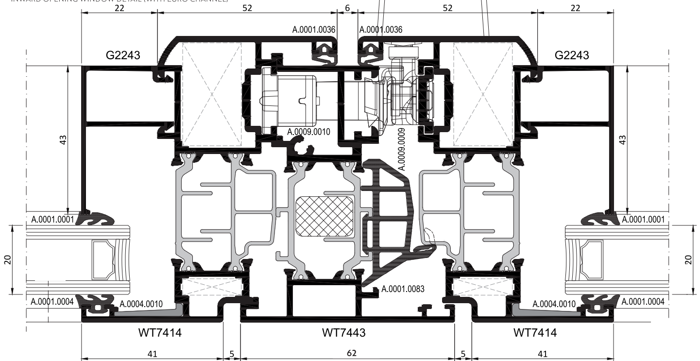
İÇE AÇILIM PENCERE DETAYI (EURO KANALLI) INWARD OPENING WINDOW DETAIL (WITH EURO CHANNEL)
