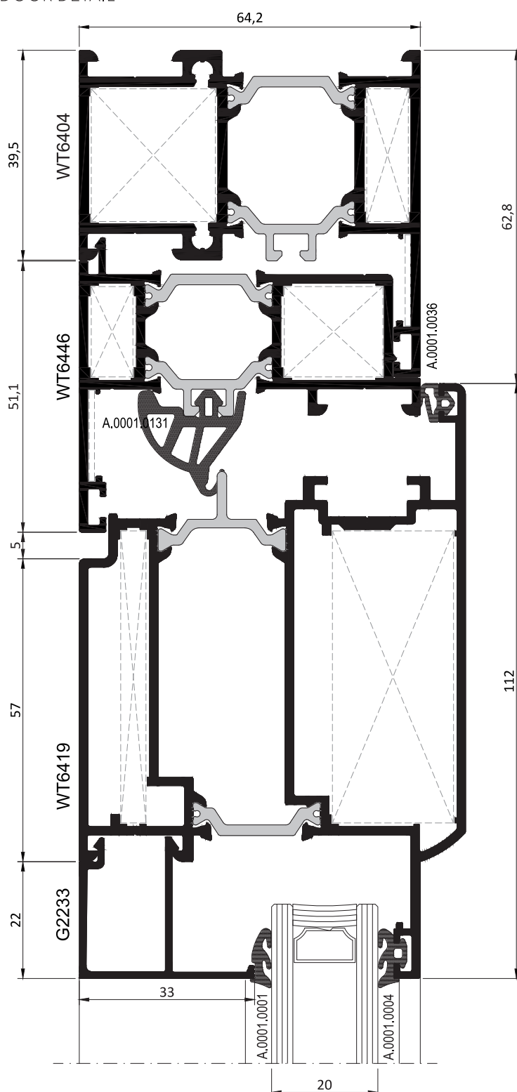
DIŞA AÇILIM BİNİLİ KAPI DETAYI OUTWARD OPENING DOOR DETAIL
