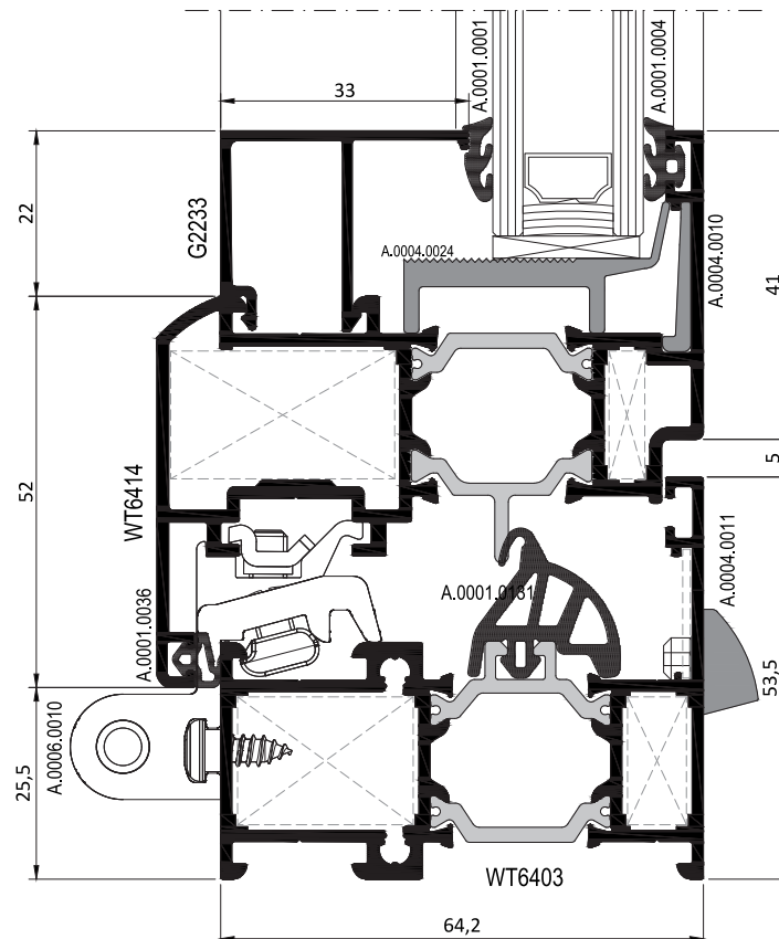
VASİSTAS AÇILIM PENCERE DETAYI BOTTOM HUNG OPENING DETAIL
