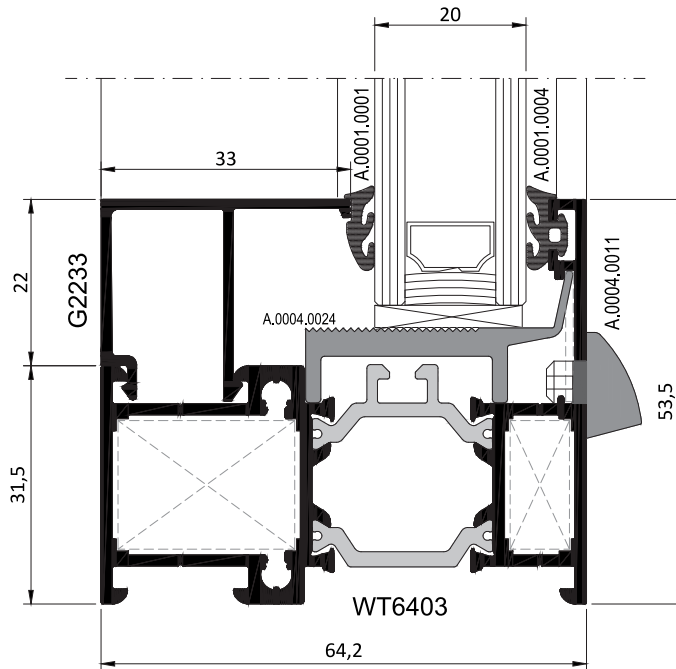
SABİT PENCERE DETAYI FIXED WINDOW DETAIL
