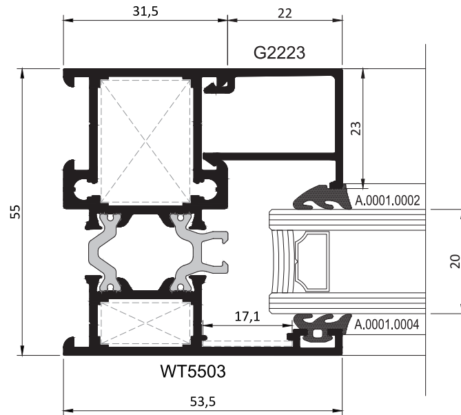
SABİT PENCERE DETAYI FIXED WINDOW DETAIL
