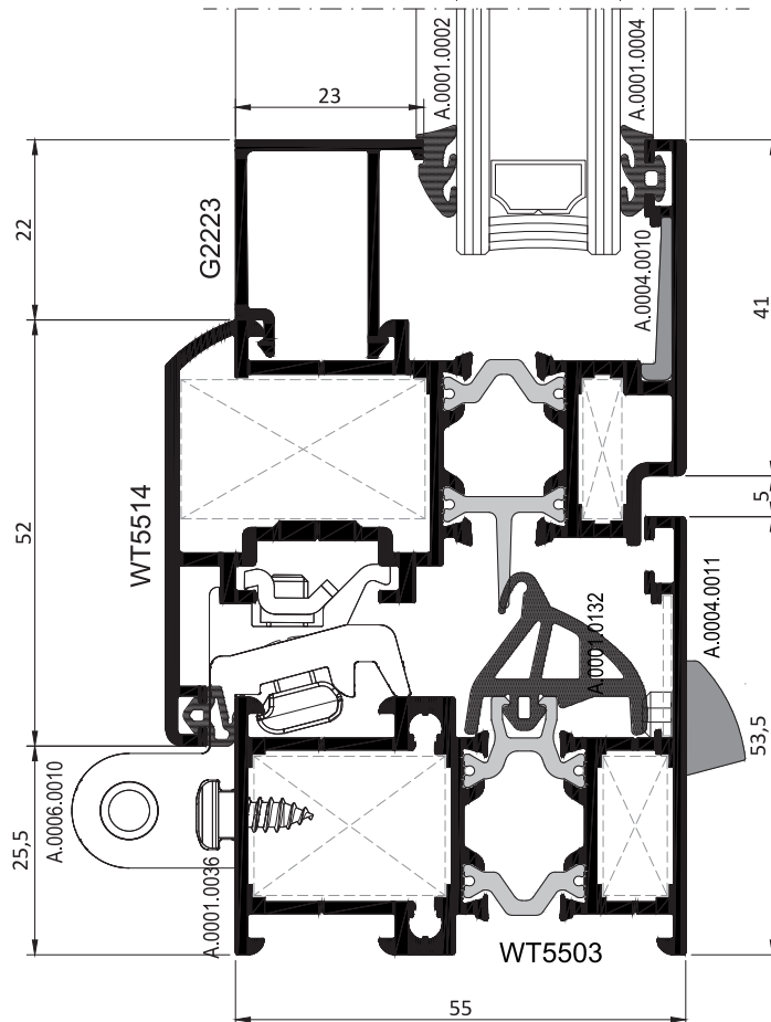
VASİSTAS AÇILIM PENCERE DETAYI BOTTOM HUNG OPENING DETAIL
