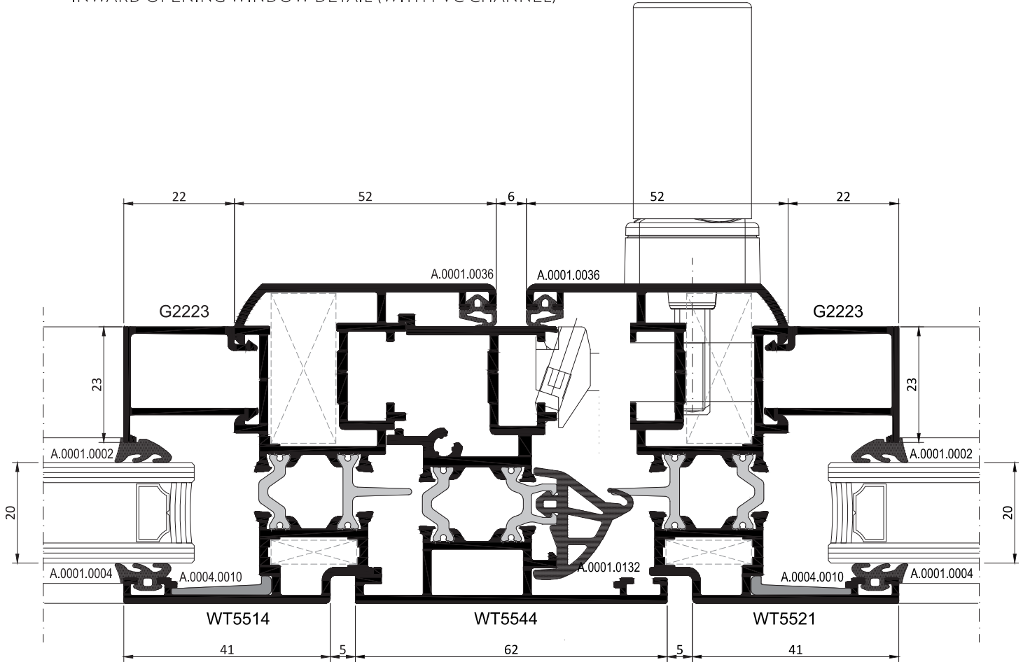
İÇE AÇILIM PENCERE DETAYI (PVC KANALLI) INWARD OPENING WINDOW DETAIL (WITH PVC CHANNEL)
