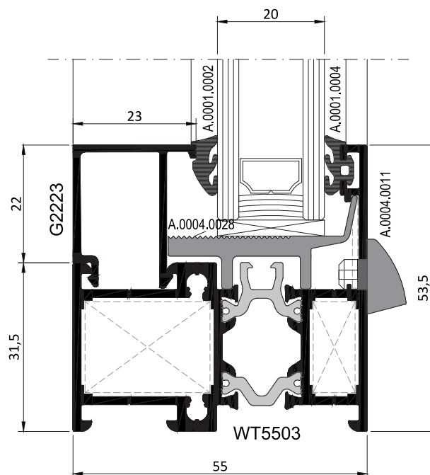
SABİT PENCERE DETAYI FIXED WINDOW DETAIL
