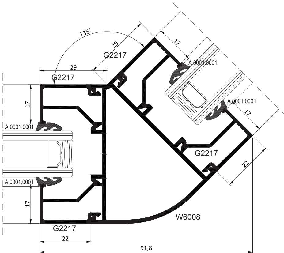
135° DÖNÜŞ 135° CORNER
