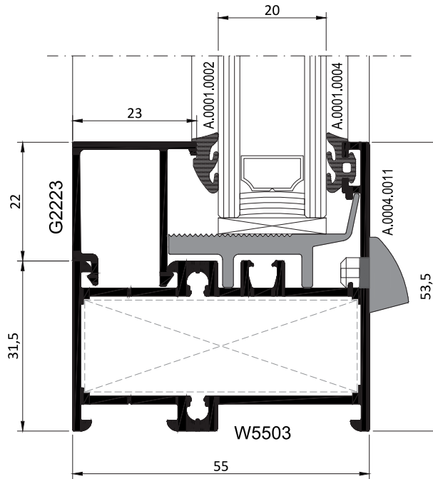
SABİT PENCERE DETAYI FIXED WINDOW DETAIL
